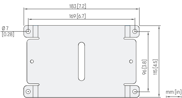
Indigo500 adapter plate dimensions
